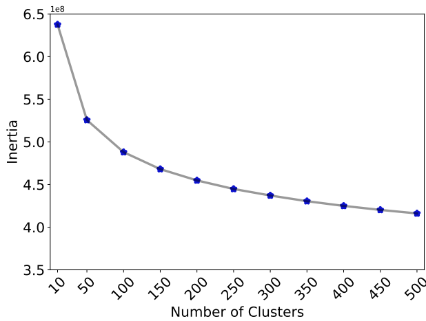
Figure 6: Elbow plot of K-means inertia as a function of the number of clusters K . The curve shows an elbow around K = 100 , after which additional clusters yield only marginal reductions in inertia.
